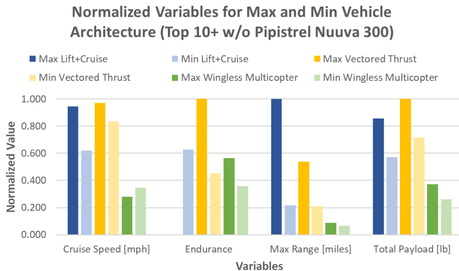
Figure 3.55. Normalized variables for max. and min. vehicle architecture (Top 10+ w/o Pipistrel Nuuva 300).
