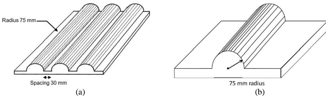
Figure 3.72. Example of a crush textured platen for modules and packs as per (a) SAE J2464 (SAE International, 2021) and (b) SAND2017-6925 (Orendorff et al., 2017).
