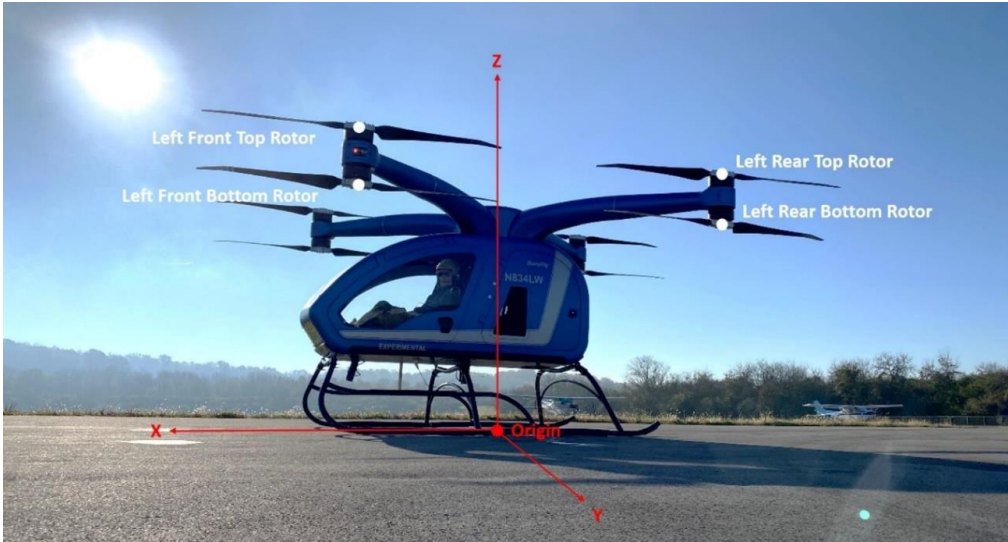
Figure 3.84 Moog “SureFly” proof-of-concept electric multi-rotor UAM (Huff et al., 2021).
