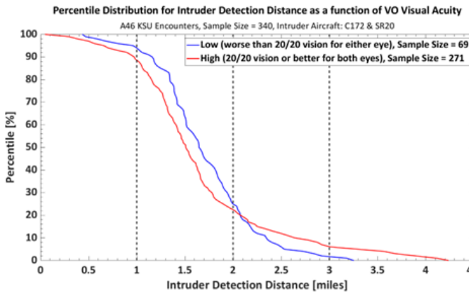
Figure 5. Percentile distribution of intruder detection distance as a function of the VO Visual Acuity categories for the KSU flight test encounters.
