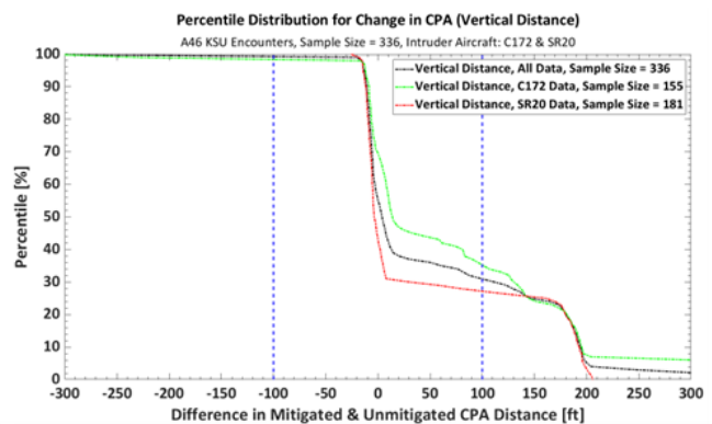
Figure 11. Percentile Distribution for Change in CPA (vertical distance) calculated for the KSU Flight Test Encounters.
