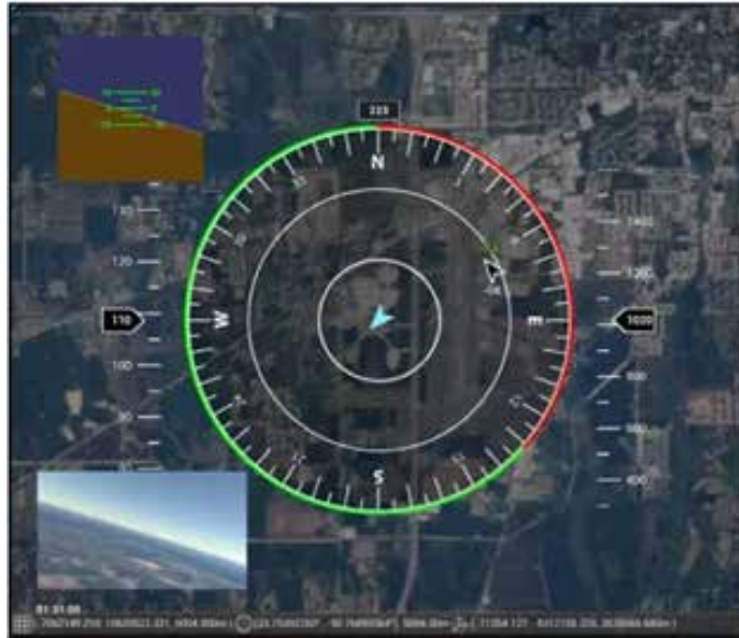
Figure 3. DAA user interface design.
