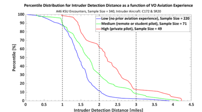
Figure 4. Percentile distribution of intruder detection distance as a function of the VO Aviation Experience categories for the KSU flight test encounters.
