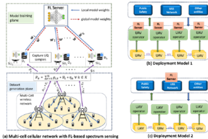
Figure 1. Federated-Learning (FL) Model for Dynamic Spectrum Monitoring (left), and Two Envisioned Deployment Models (right).
